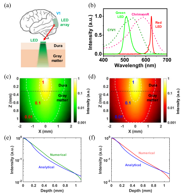
Fig. 2. (a) Optical model showing optogenetic stimulation of the human visual cortex (V1) with surface mounted micro-LEDs. (b) Absorption spectra of ChromsonR and C1V1, and emission spectra of red and green micro-LEDs. (c) and (d) Normalized light intensity distribution profiles on a cross-sectional plane along the propagation direction based on numerical simulation at wavelengths of (c) 530 nm and (d) 620 nm. (e) and (f) Normalized light intensity profiles at varied depths along the propagation direction at (e) 530 nm and (f) 620 nm.
